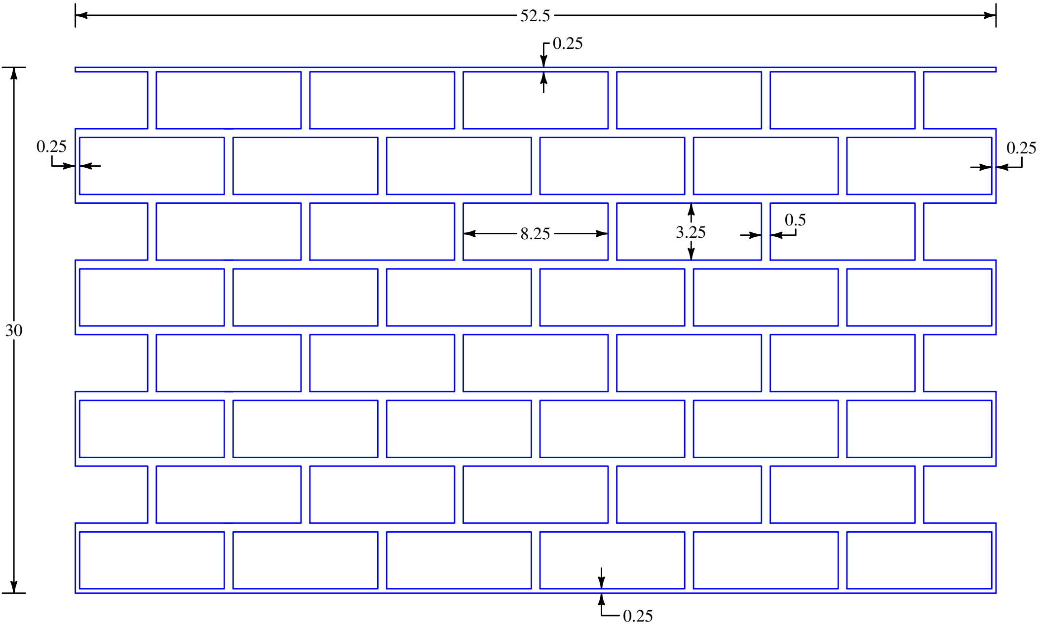
RUNNING BOND BRICK
